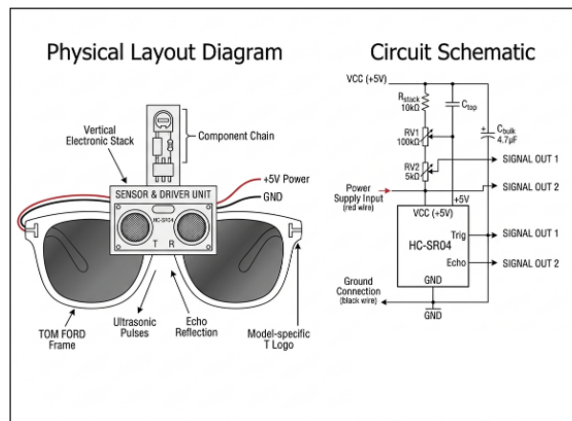
Figure 6. Physical layout prototype diagram/Circuit schematic.
